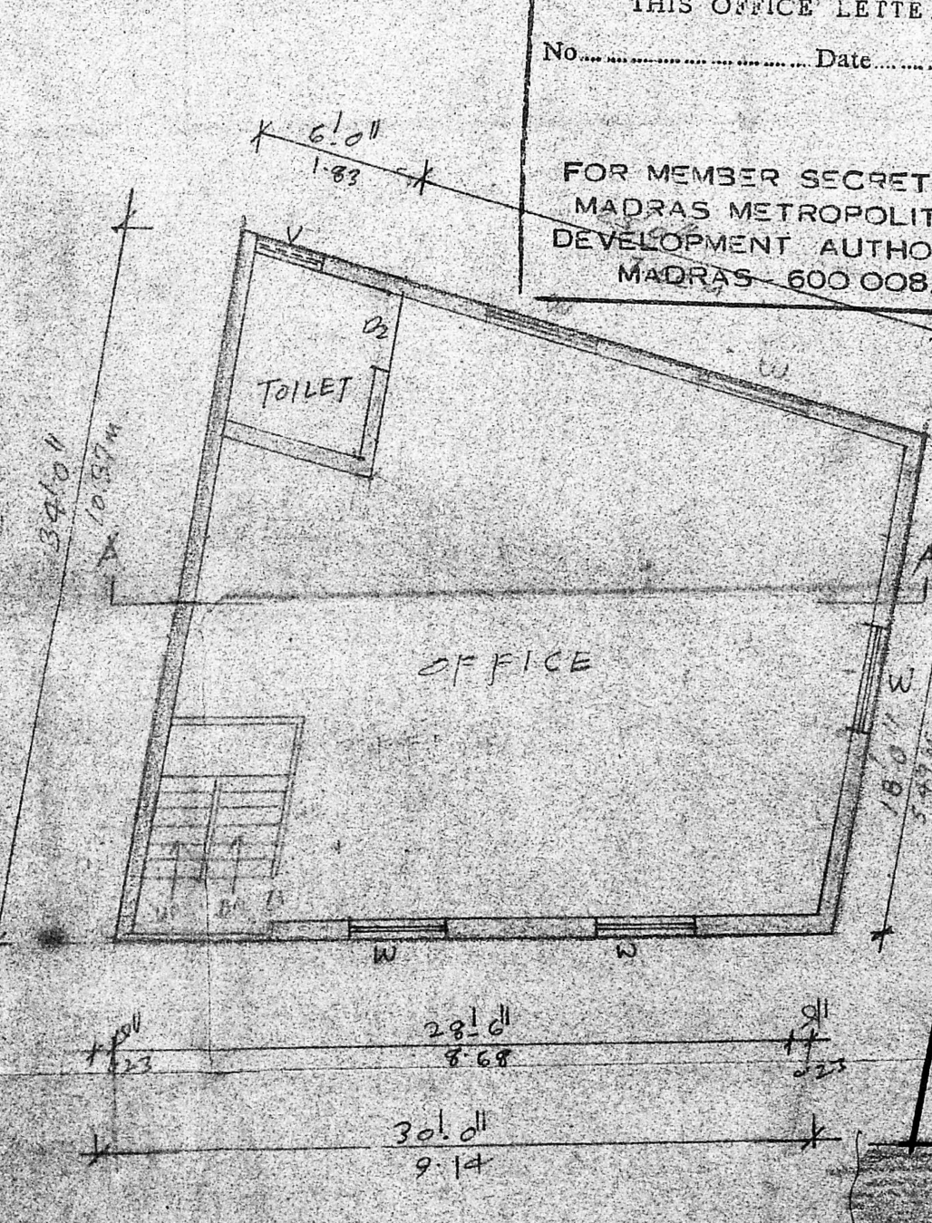
TYPICAL FLOOR PLAN (FIRST AND SECOND FLOOR)
